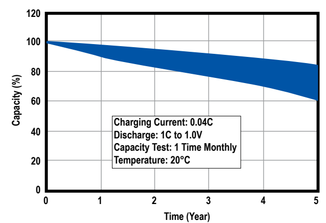
Cycle Life Using Trickle Charging
